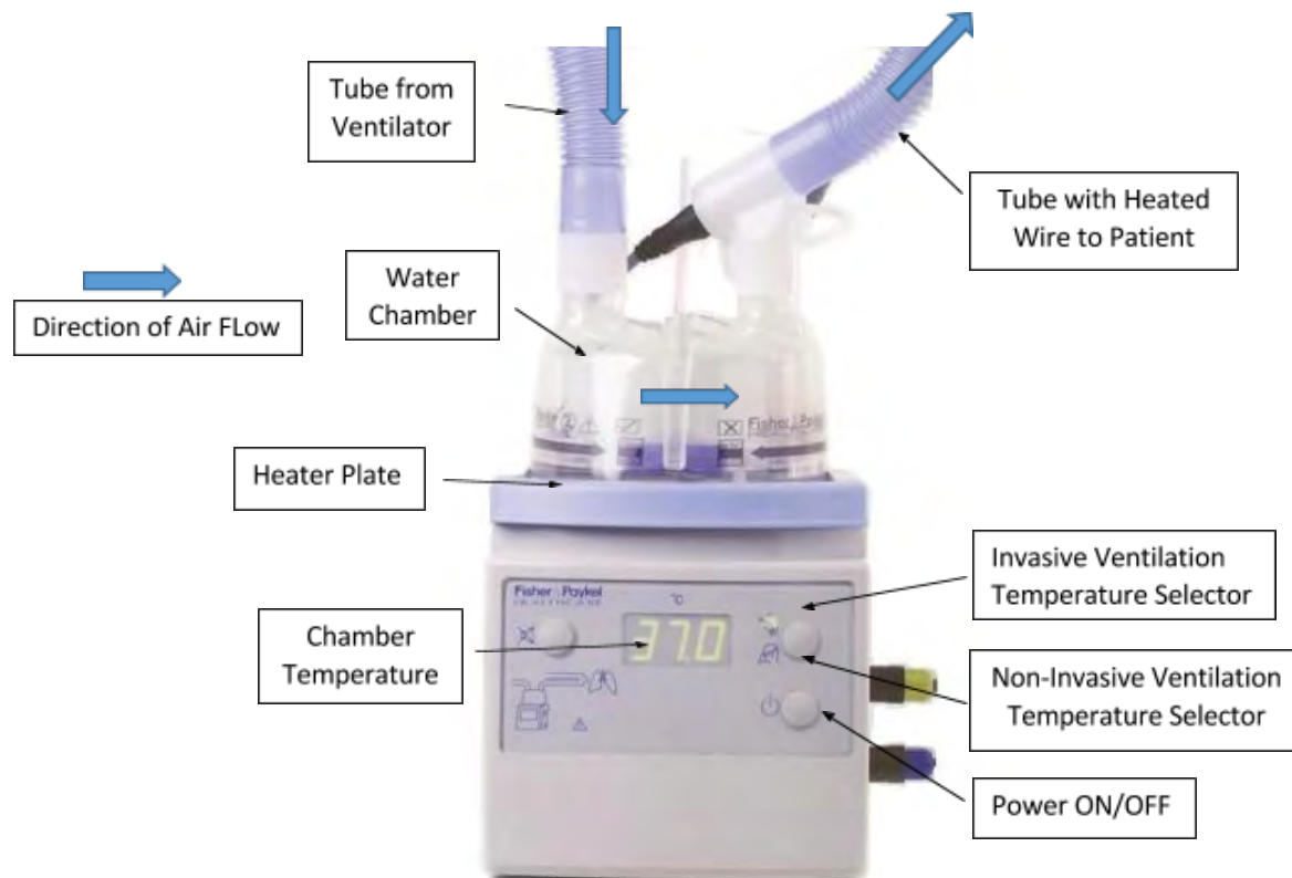
Figure 6. Fisher and Paykel MR850 Humidifier http://bemeseast.com/index.php?route=product/product&product_id=180
